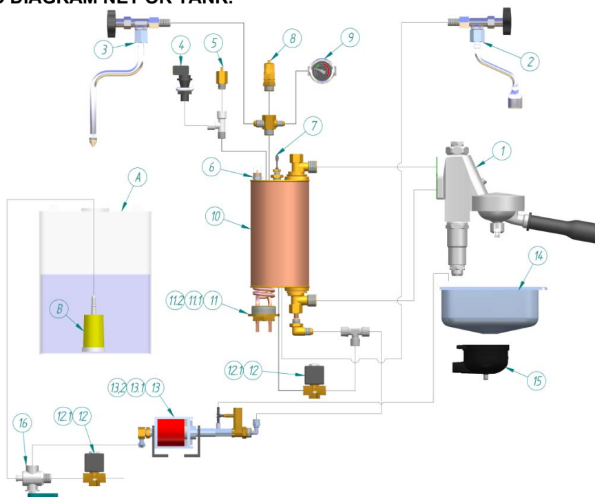
HYDRAULIC DIAGRAM NET OR TANK.
