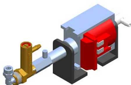
TANK CONNECTION.
