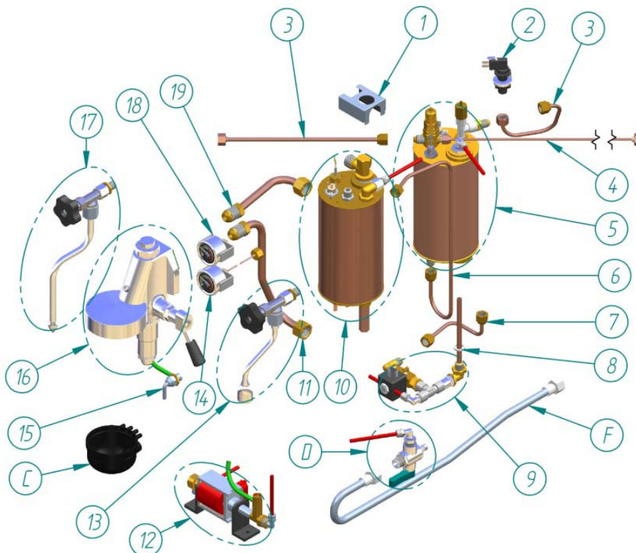
OFFICE LEVA MULTIBOILER WATER NETWORK CONNECTION.
